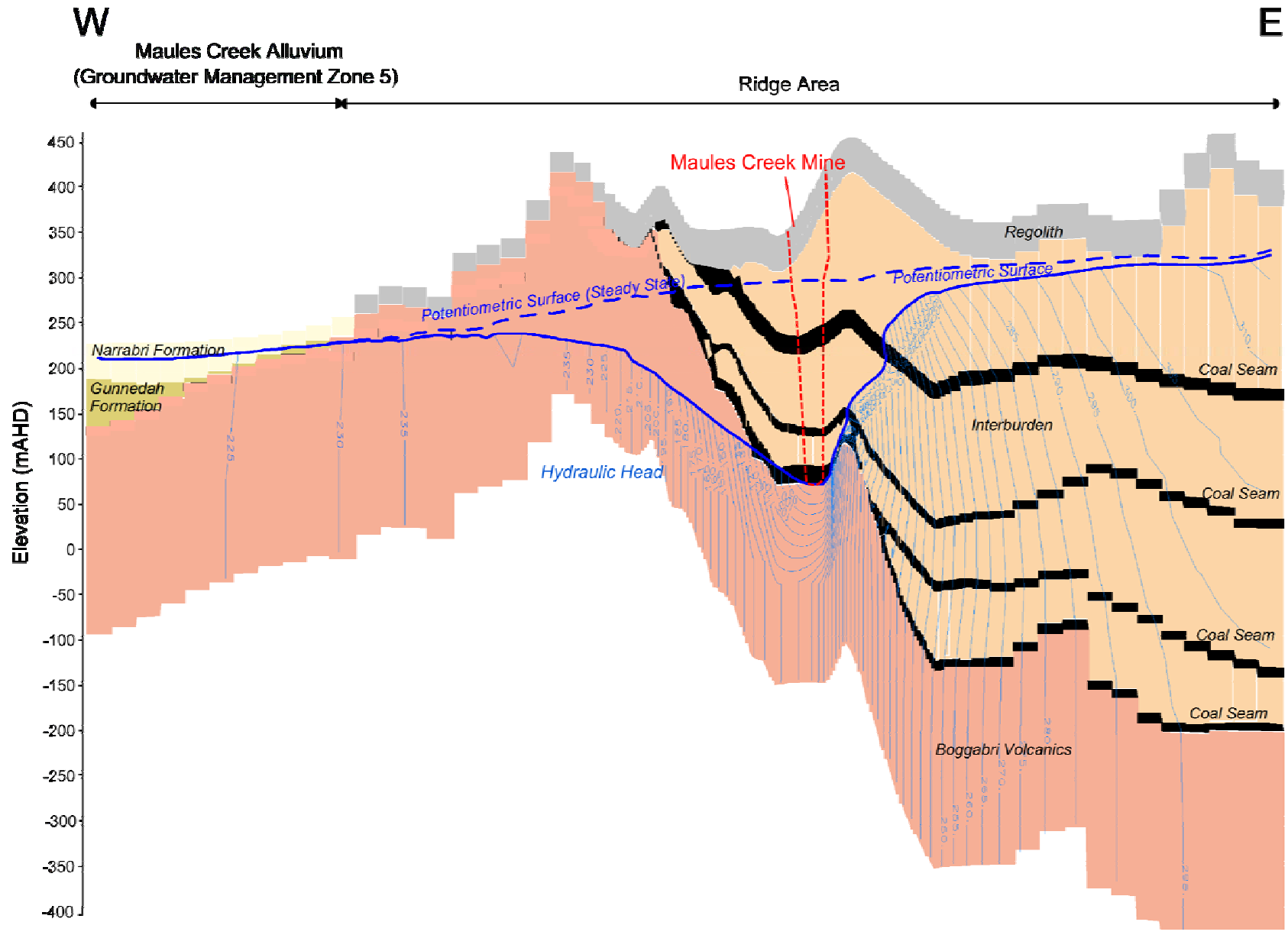
Cross Section A4.14 - W-E - Groundwater Levels - Year21
