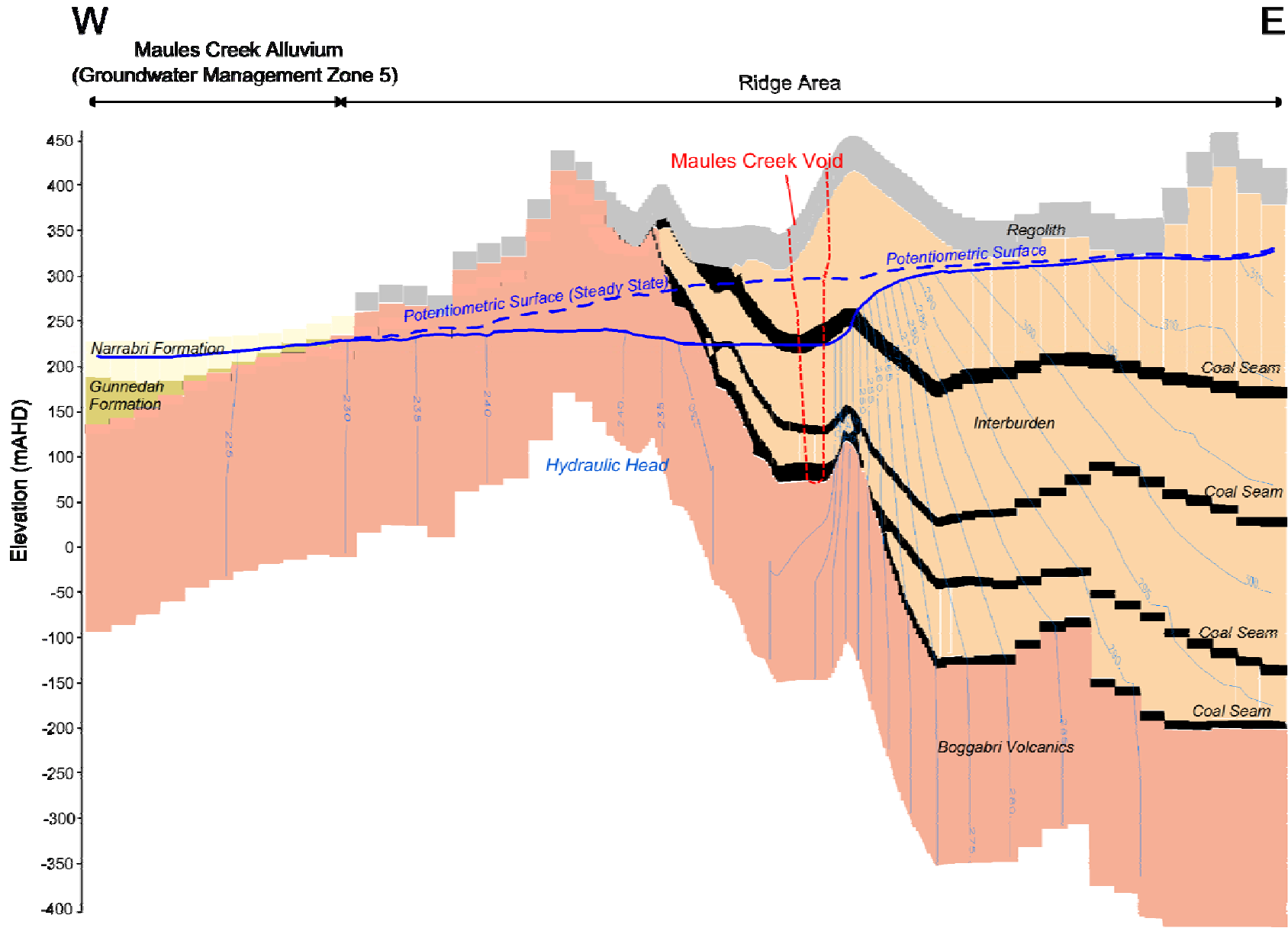
Cross Section A4.15 - W-E - Groundwater Levels - Recovered Heads with Void
