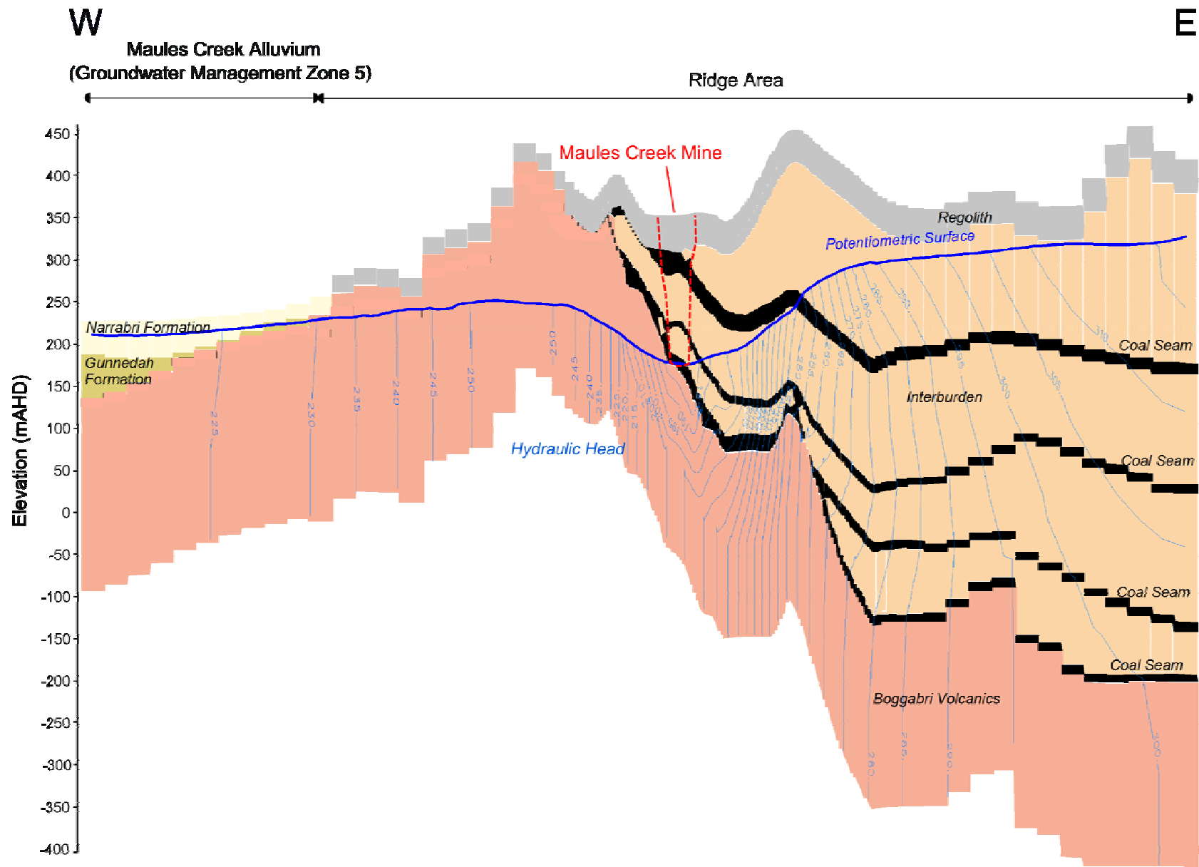
Cross Section A4.12 - W-E - Groundwater Levels - Year 10
