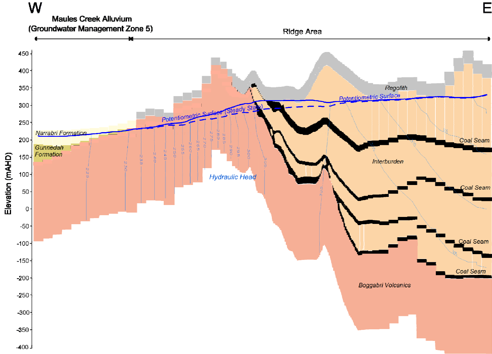
Cross Section A4.16 - W-E - Groundwater Levels - Recovered Heads with Backfill
