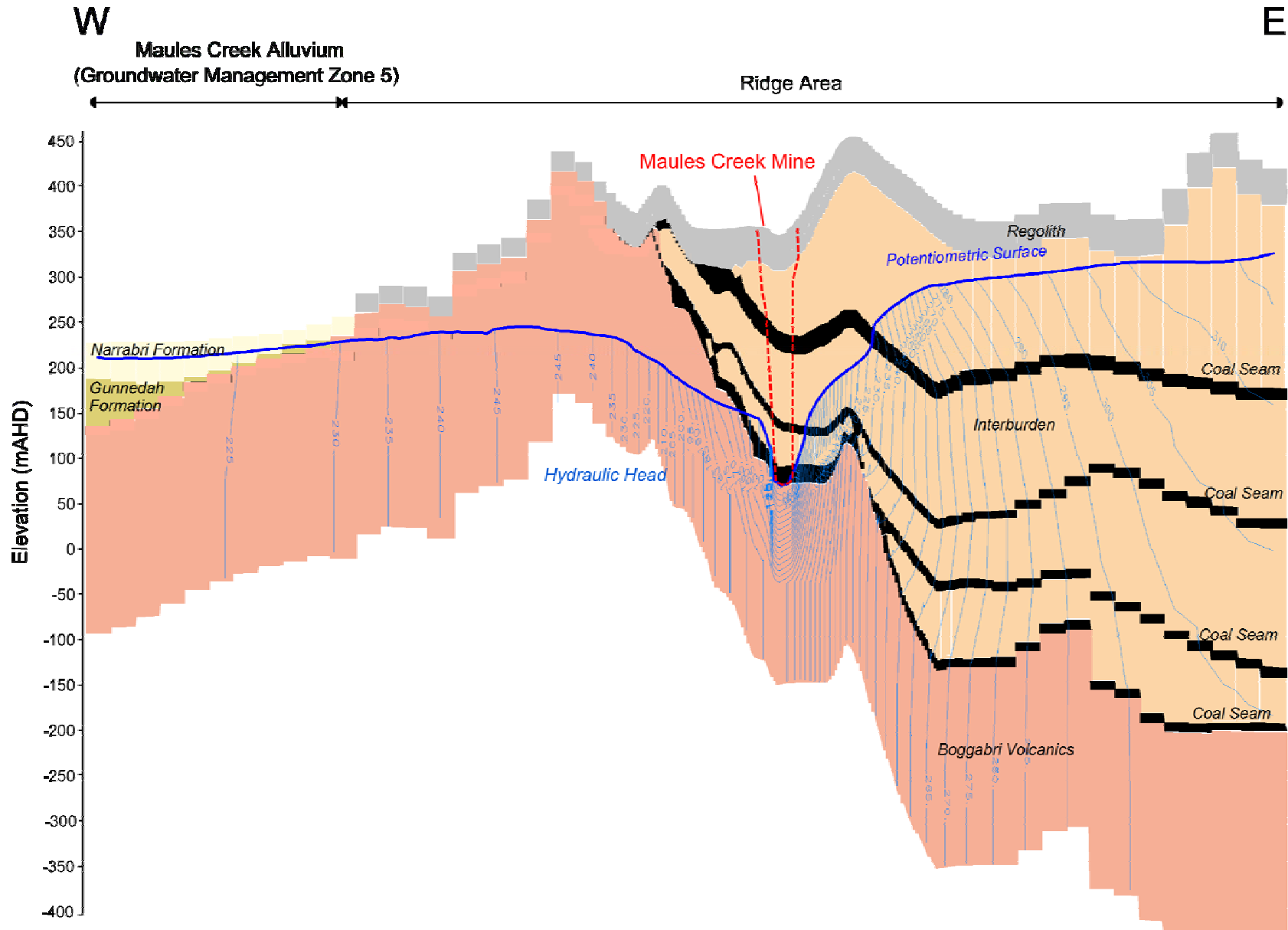
Cross Section A4.13 - W-E - Groundwater Levels - Year 15
